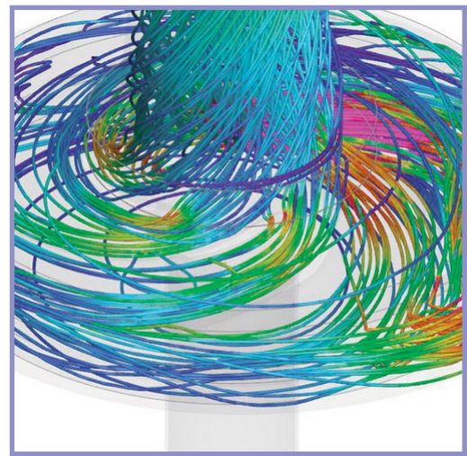
Wind-Milling and Thrust Bearing Performance Analysis for Multi-Pump Nuclear Test Loop
