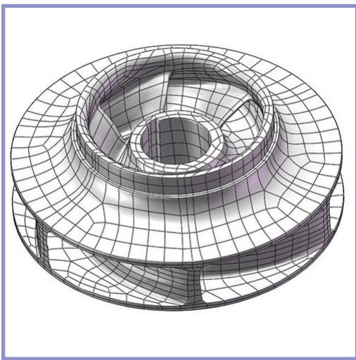
Advanced Scanning and Computational Fluid Dynamic Analysis on Safety Related Impeller
